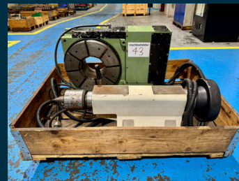
Lot 43: MATSUMOTO MMK 400 4th Axis Attachment with Tailstock
