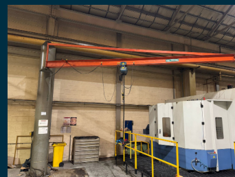
Lot 216: UNKNOWN MFR 500Kg SWL Jib Crane with Electric Hoist
