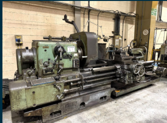
Lot 17: DEAN SMITH & GRACE Type 25 x 72" (1828mm) Straight Bed Centre Lathe
