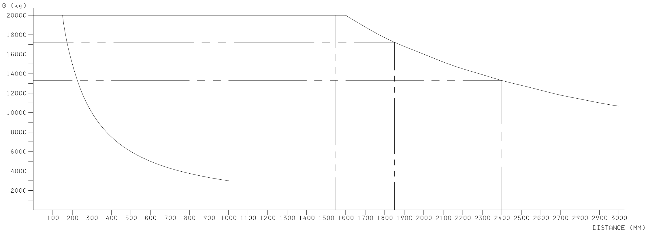
LOAD DIAGRAM SP/E 40000
